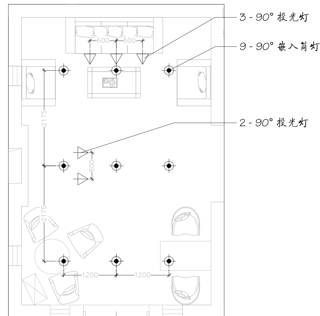
1 1F-(1-D) Light Plot 1:75
